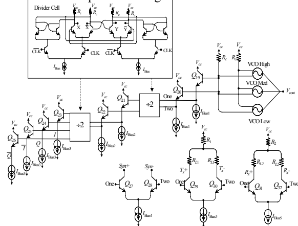
Fig. 4. System Level Circuit diagram for the VCO.
