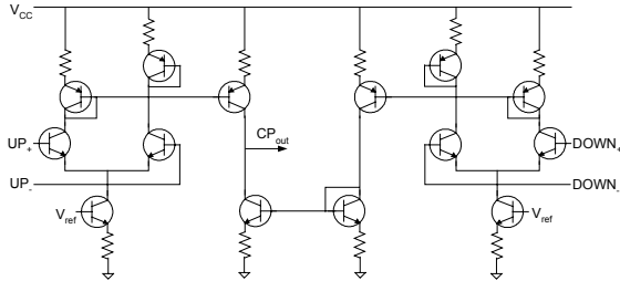
Fig. 6 Differential charge pump circuitry.
