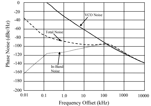
Fig. 7. Optimum Crossover Point (150kHz).
