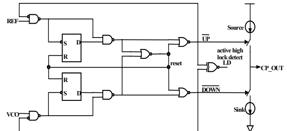
Fig. 2. Dead-zone-free phase frequency detector with differential charge pump.
