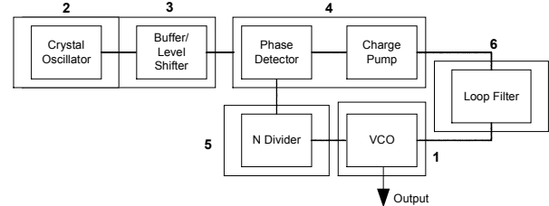
Fig. 5. PLL noise sources partitioning.
