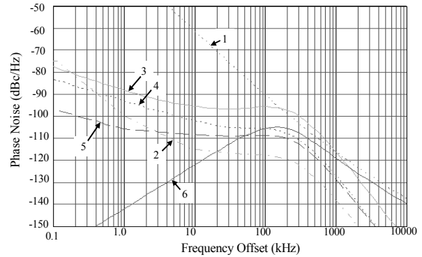
Fig. 6. PLL Noise Contributors.
